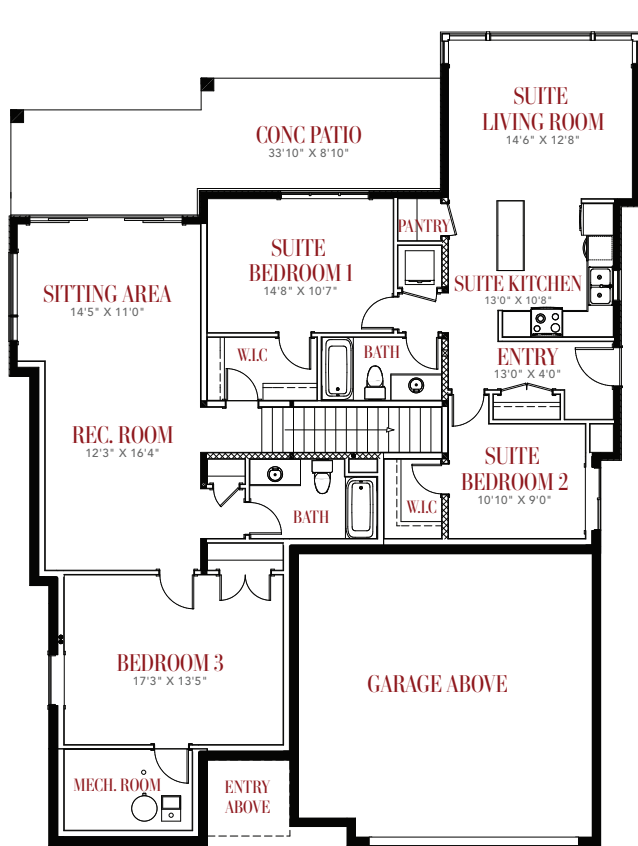
GROUND FLOOR 1815 SQ. FT.
