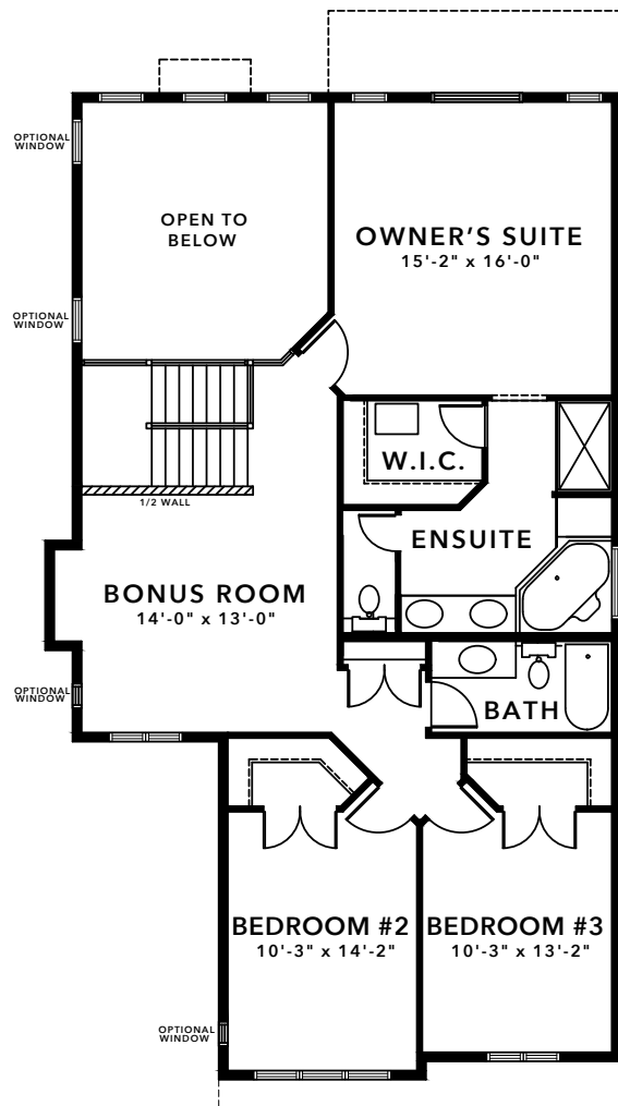
UPPER FLOOR 1220 sqft
