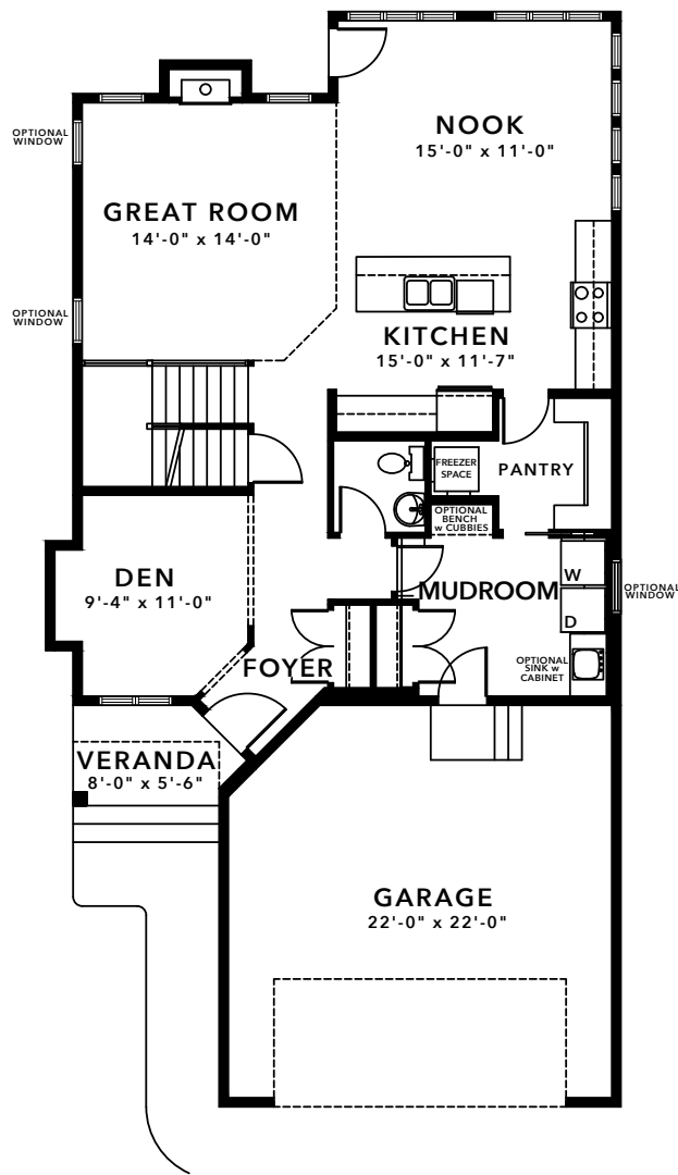
MAIN FLOOR 1098 sqft
